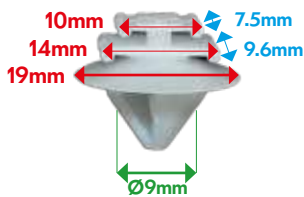
VB17105 FASTENER FOR MOULDING
