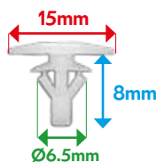
VB4000713 FASTENER WATERPANEL / INNER PANEL
