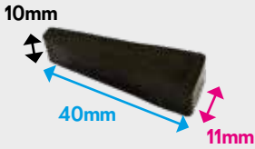
VB4000701 RUBBER WEDGE 100/A6 (91-97)
