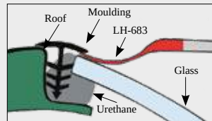
"CHRISTMAS TREE" MOULDING REMOVER can easily be inserted under the moulding, does not damage the profile. The curvature guarantees the leverage effect to remove the clips.
