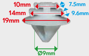
VB17105 FASTENER FOR MOULDING Saxo, Berlingo, Evasion, C3, C2, Jumpy III
