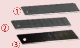
① BLADE (NOT SNAP-OFF) package of 10 - for L2 and XL2 110x18x0.5mm - 65g
