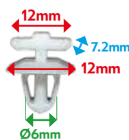
VB12029 WINDSHIELD SCUTTLE Berlingo et Partner
