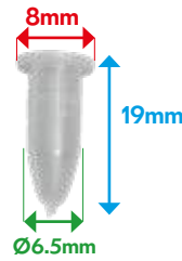
VB89427 TRIM CLIP BUSH
