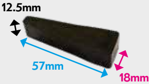
VB4000501 RUBBER WEDGE
