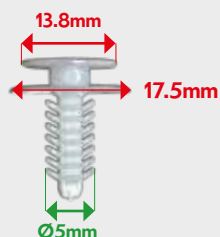
VB59405 TRIM CLIP various models
