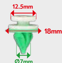
VB56405 TRIM CLIP Laguna II
