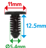
VB4000715 FASTENER WATERPANEL / INNER PANEL
