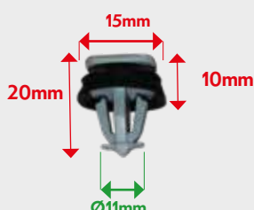
VB4000910 SIDE WINDSHIELD CLIP Daily III
