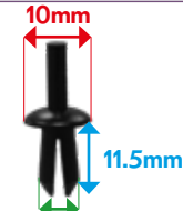
VB4000709 FASTENER WATERPANEL / INNER PANEL
