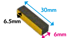
VB4000409 SELF-ADHESIVE SPACER C4 (04-10)
