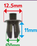
VB4000706 FASTENER WATERPANEL / INNER PANEL
