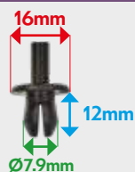
VB4000705 FASTENER WATERPANEL / INNER PANEL
