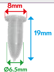
VB89427 TRIM CLIP BUSH AX, BX, Xantia, XM
