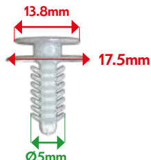
VB59405 TRIM CLIP
