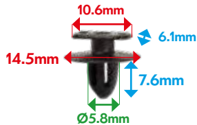
VB4000714 FASTENER WATERPANEL / INNER PANEL
