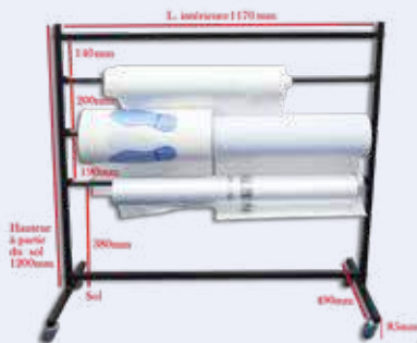
TRIPLE MOBILE DISPENSER ON WHEELS with 4 rotating wheels, 3 storage levels, holds rolls of seat covers, floor mats, wiper spools... Supplied without consumables
