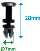
VB6407002E FASTENER Transit IV
