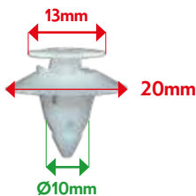
VB72155 FASTENER FOR MOULDING KA
