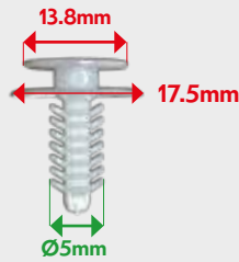
VB59405 TRIM CLIP
